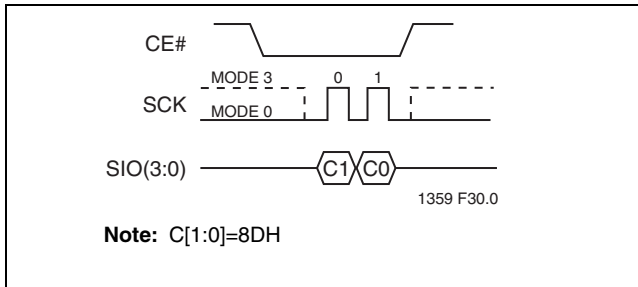
FIGURE 24: Lockdown Block-Protection Register
