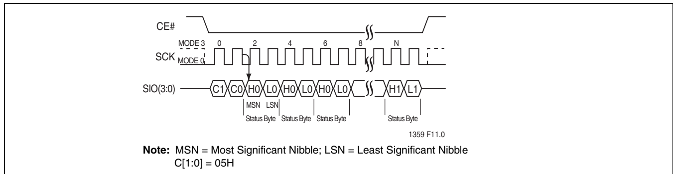
FIGURE 19: Read-Status-Register (RDSR) Sequence
