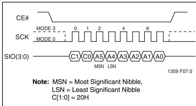
FIGURE 15: 4 KByte Sector-Erase Sequence
