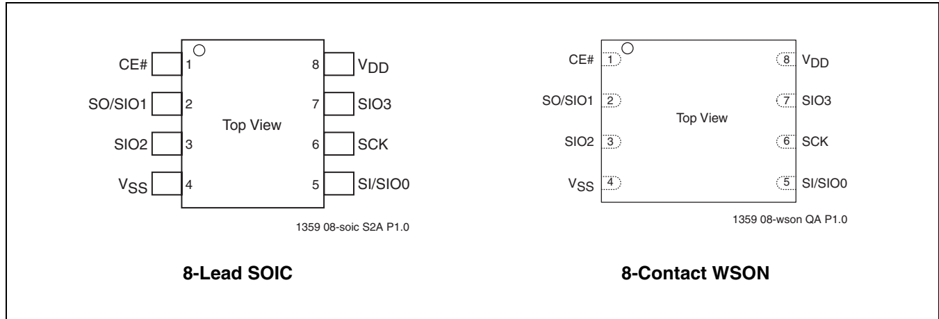
FIGURE 2: Pin Description for 8-lead SOIC and 8-contact WSON
