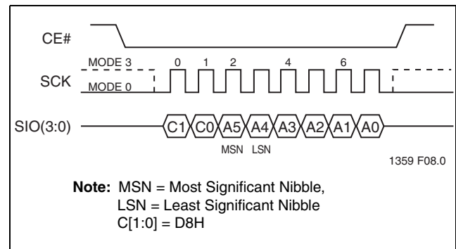
FIGURE 16: Block-Erase Sequence
