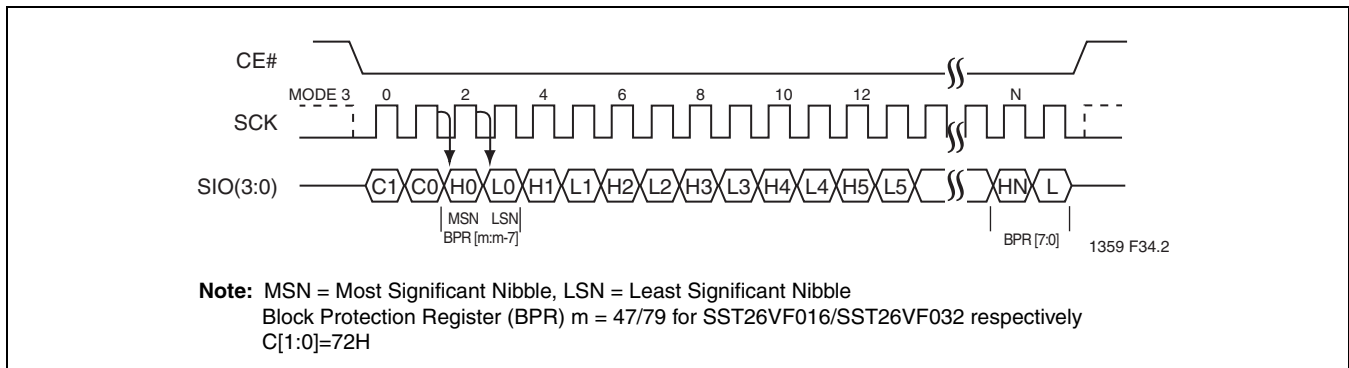
FIGURE 22: Read Block Protection Register Sequence
