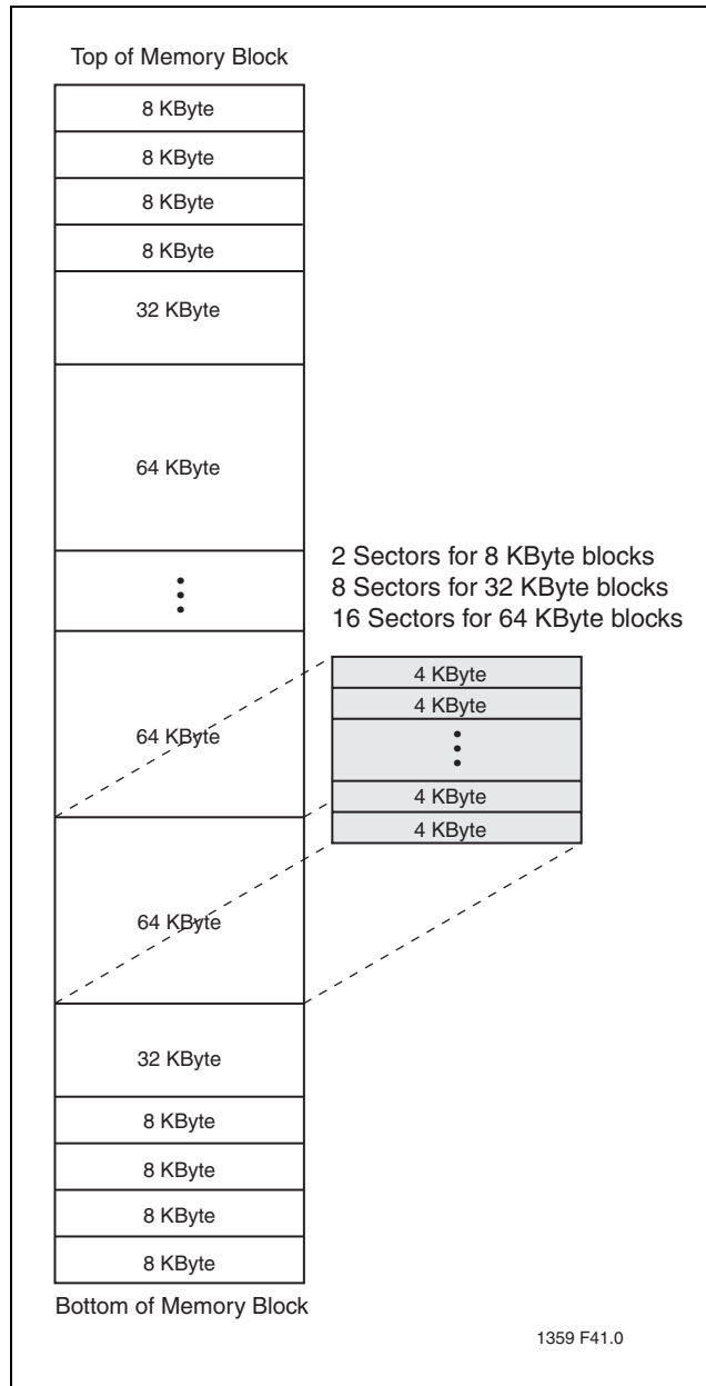
FIGURE 3: Memory Map
