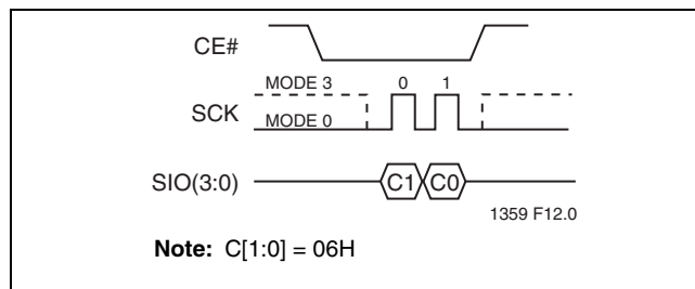
FIGURE 20: Write-Enable Sequence
