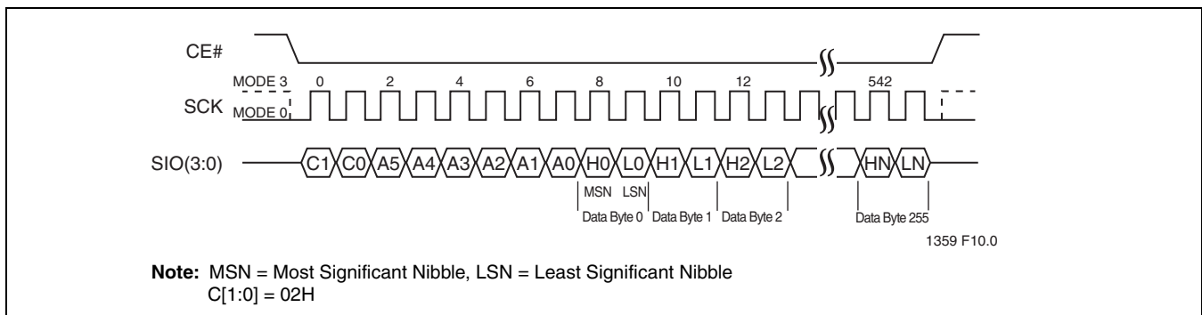
FIGURE 18: Page-Program Sequence
