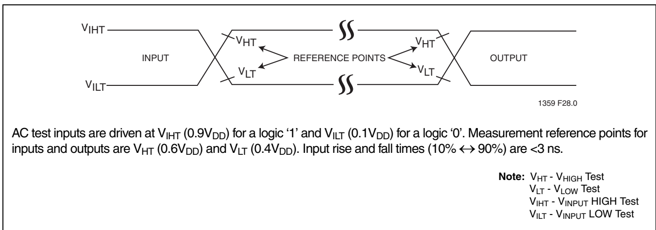
FIGURE 29: AC Input/Output Reference Waveforms
