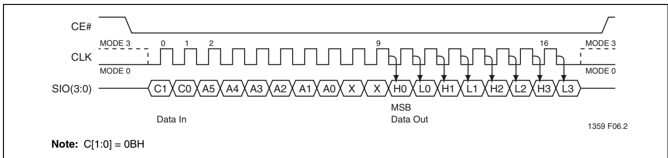
FIGURE 11: High-Speed Read Sequence (SQI)
