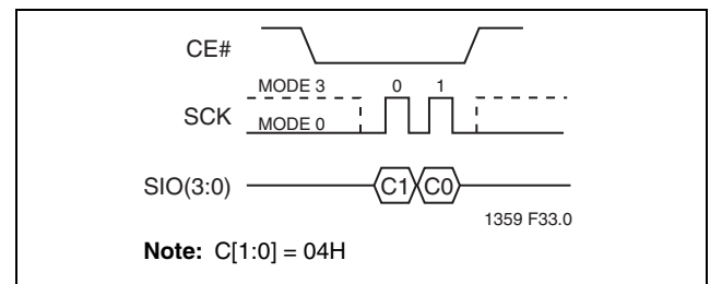
FIGURE 21: Write-Disable (WRDI) Sequence
